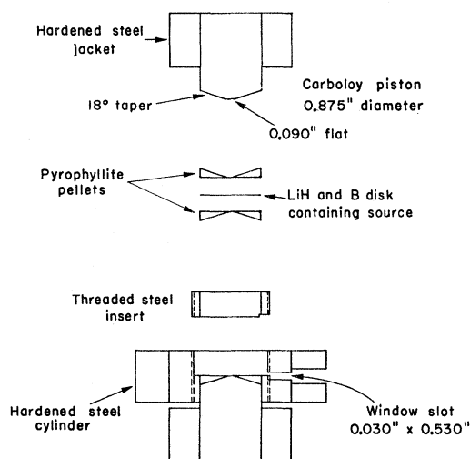
FIG. 2. Pressure cell cross section.
